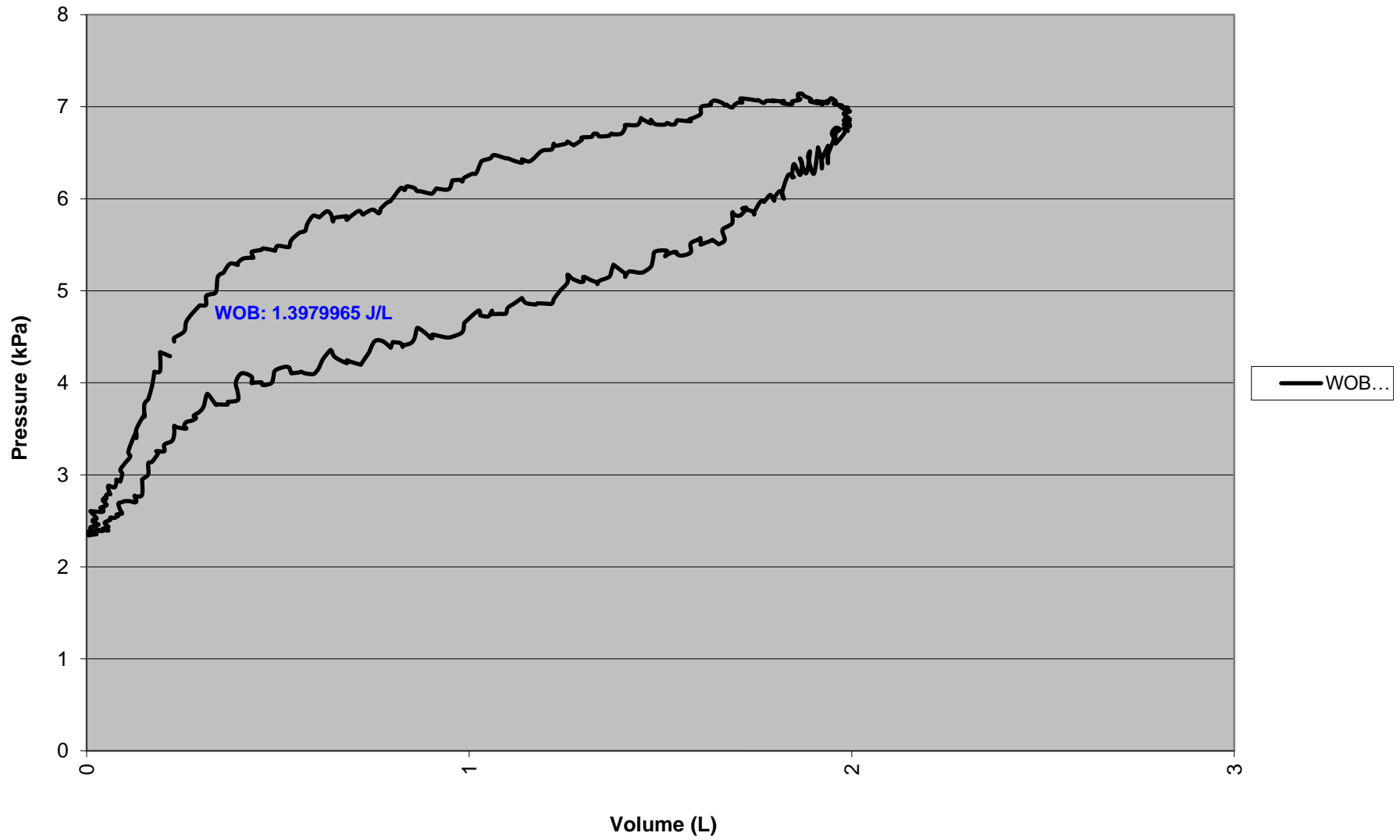
WOB Chart 1
